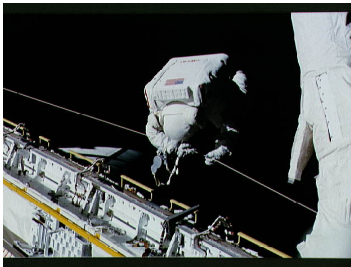
TOP: STS037-52-013 1991-04-11 Apt/MS, suited in Extravehicular Mobility Unit (EMU), tests Crew and Equipment Translation Aid (CETA) electrical hand pedal cart during EVA in P/L Bay).
