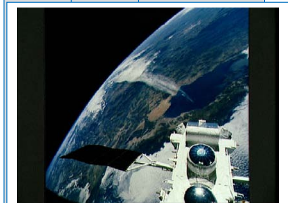
STS037-99-089 1991-04-11 Deployed Gamma Ray Observatory (GRO) over Baja California, Mexico (31.5N, 113.0W), the Salton Sea and Imperial Valley region of California where the mouth of the Colorado River empties into the Sea of Cortez are clearly visible.
